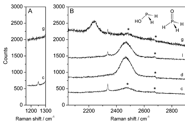
Figure 4. Raman spectra measured in the 1150–1300 \text{cm}^{-1} (A) and in the 2100–2800 \text{cm}^{-1} (B) frequency ranges on a transparent area (trace d) and on several bubbles (traces c, l, and g). See Figure 1 B for the label matching with the sample zones. The sharp band at 2330 \text{cm}^{-1} is due to the P–H stretching vibration of \text{PH}_3 . The bands at 1250 and 2470 \text{cm}^{-1} have been assigned to the P=O and P–H stretching of \text{H}_3\text{PO} , whereas the band at 2236 \text{cm}^{-1} has been assigned to the P–H stretching of \text{PH}_2\text{OH} . The asterisks indicate Raman signals from the diamond anvils.
