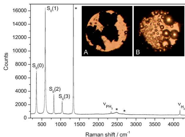
Figure 5. Images of a sample at 0.6 GPa and 298 K taken before (A) and after (B) irradiation (350 nm, 500 mW, 5 h) and Raman spectrum measured on a bubble from (B). The rotational bands of \text{H}_2 ( S_0(i) with i=0,1,2,3 ) and the vibrations of \text{H}_2 and \text{PH}_3 are the only observed bands. The asterisks indicate Raman signals from the diamond anvils of the DAC.
